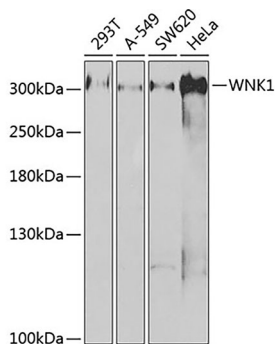
Fig. 1. Western blot analysis of extracts of various cell lines, using WNK1 antibody at 1:1000 dilution. Secondary antibody: HRP-labeled Goat Anti-Rabbit IgG(H+L) (A0208) at 1:1000 dilution. Lysates/proteins: 25μg per lane. Blocking buffer: QuickBlock™ Blocking Buffer (P0231). Detection: BeyoECL Star (P0018A). Exposure time: 1s.
